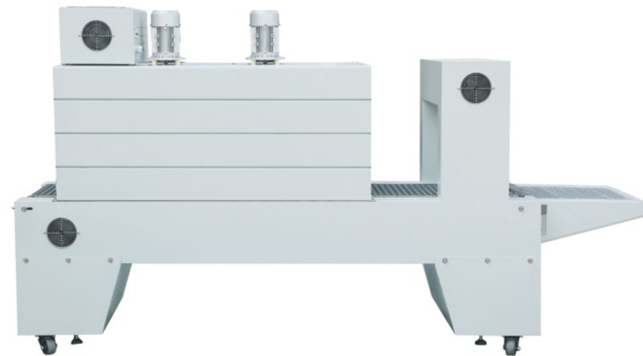
BSE5040A/BSE6040A PE Film shrink packaging machine (Hotair circulation, Jet model) PE膜熱收縮包裝機
