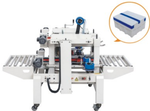
DFXA5030C Carton sealer (Top & side tapping) 膠帶封箱機
