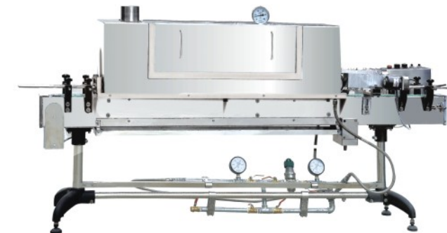
ZBS83A Steam label shrink machine 蒸汽標籤收縮機
