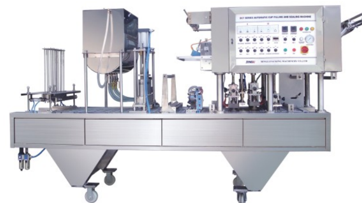
CFD-4 Automatic cup filling and sealing machine (Four cups) Pneumatic type for big capacity
