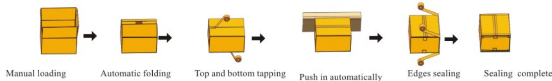
FXZ5050 Auto folding carton sealer & DFXS7050 Automatic carton edges sealer
